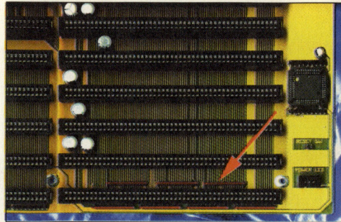
This is the problem connection on Elbox's A4000 Zorro 3 expansion.
