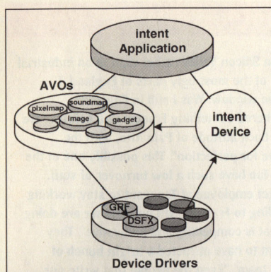
The intent windowing toolkit manages objects like windows and gadgets.
